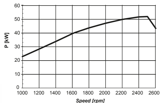
4.63H Yanmar 4TNV98C 53 kW - 72 HP
